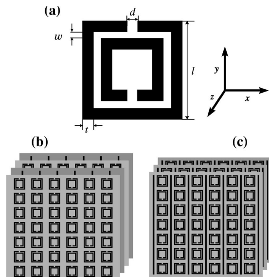
FIG. 1. (a) A single SRR with parameters \ell=3 mm and d=t=w=0.33 mm. (b)–(c) Schematic drawing of two different configurations of the composite medium consisting of thin wires and SRRs.
